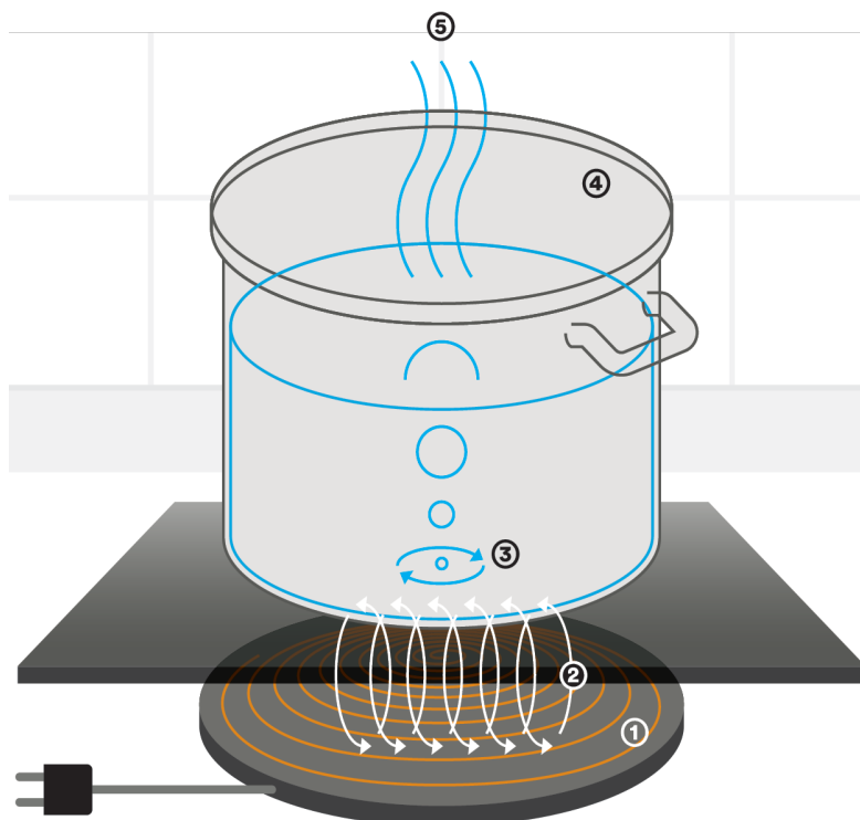
Figure 1: Alternating electric current in the power coil 1 produces a fluctuating electromagnetic field 2 . This field in turn generates small electrical currents 3 in the bottom of the pot. These currents encounter resistance in the metal of the cookware 4 which creates heat 5 .
