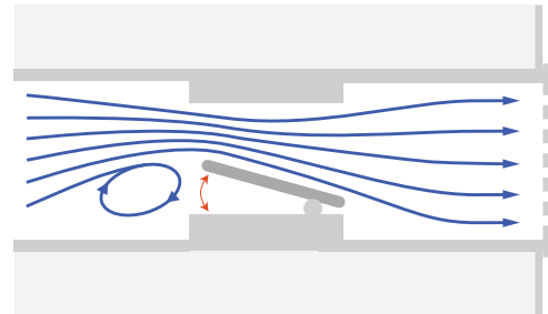
Fig 2. A Constant Airflow Regulator (CAR) automatically dampers airflow to achieve consistent ventilation.
