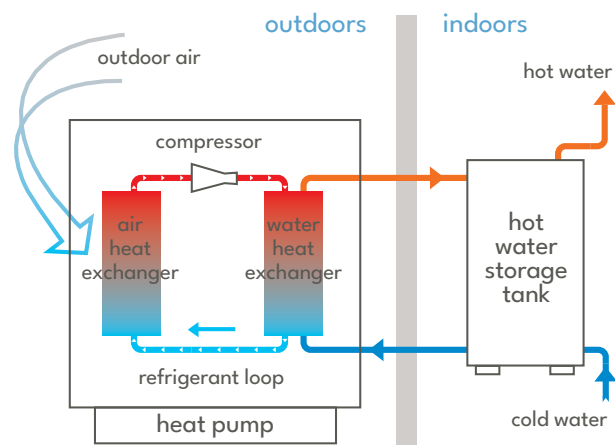
Fig 1. Heat from outdoor air is drawn into the AWHP and is absorbed by a refrigerant. As the refrigerant passes through the compressor, its pressure and temperature rises. The refrigerant then passes through the water heat exchanger to heat the domestic supply water, which is pumped to the storage tank for distribution.
